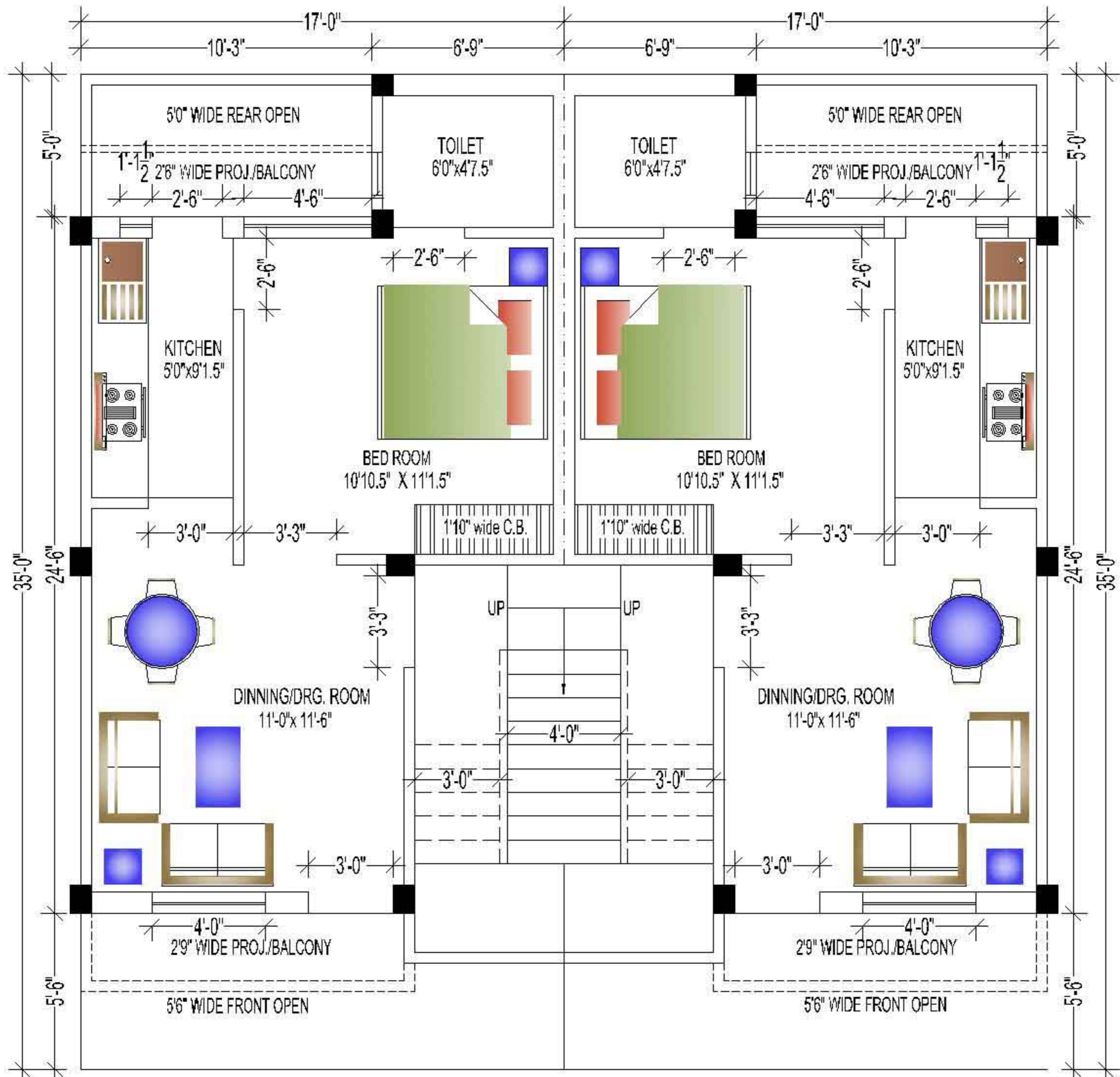
TITLE:-GROUND FLOOR PLAN
